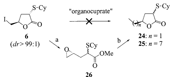
Scheme 7. Reagents and conditions: (a) \text{K}_2\text{CO}_3 , MeOH, room temp., 96%, dr 1:1; (b) \text{RMgBr} , CuI, THF, 0 °C, R = Me (70%, dr 7:3), R = Heptyl (22%, dr 99:1).
