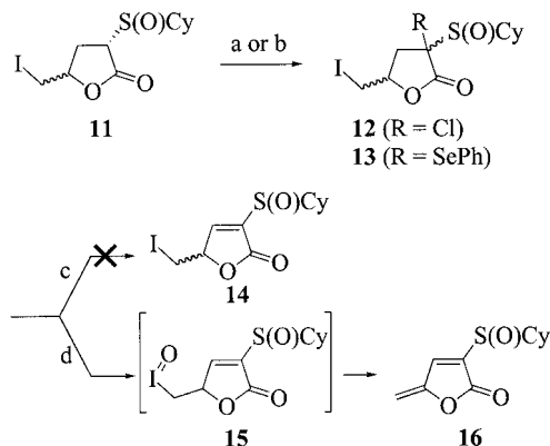
Scheme 4. Reagents and conditions: (a) NCS, \text{K}_2\text{CO}_3 , \text{CH}_2\text{Cl}_2 , 98%; (b) LDA, THF, -78^{\circ}\text{C} , then PhSeCl, 53%; (c) LiBr or \text{Li}_2\text{CO}_3 or \text{NEt}_3 ; (d) m -CPBA or \text{H}_2\text{O}_2 , \text{K}_2\text{CO}_3 or pyridine, \text{CH}_2\text{Cl}_2 , room temp., 90%.
