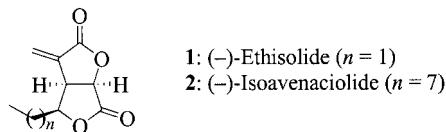
Scheme 1. Structure of the bis(lactone)s.
