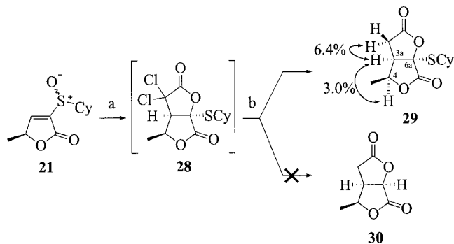
Scheme 9. Reagents and conditions: (a) \text{CCl}_3\text{COCl} , Zn-Cu, THF, 10 min, 0 °C; (b) \text{Bu}_3\text{SnH} , AIBN, toluene, 110 °C, 40% (2 steps).
