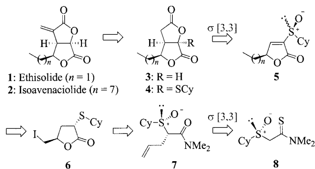
Scheme 2. Retrosynthetic analysis.
