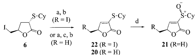
Scheme 6. Reagents and conditions: (a) m -CPBA, \text{CH}_2\text{Cl}_2 , 0^{\circ}\text{C} , 95%; (b) TFAA, \text{CH}_2\text{Cl}_2 , 0^{\circ}\text{C} , 93%; (c) \text{Bu}_3\text{SnH} , AIBN, THF, 65^{\circ}\text{C} , 97%; (d) m -CPBA, \text{CH}_2\text{Cl}_2 , 0^{\circ}\text{C} , 98%.
