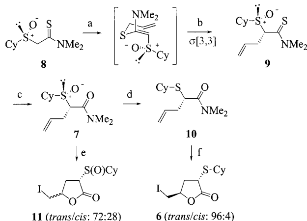
Scheme 3. Reagents and conditions: (a) t BuLi, THF, -40^{\circ}\text{C} , then allyl bromide; (b) \text{CeCl}_3 (10%), THF, room temp., 20 h; (c) dimethyldioxirane (formed in situ), 69% overall, dr 99:1; (d) \text{P}_4\text{S}_{10} , \text{CH}_2\text{Cl}_2 , room temp., 90%; (e) \text{I}_2 , THF/ \text{H}_2\text{O} , 60%; (f) \text{I}_2 , THF/ \text{H}_2\text{O} , 98%.
