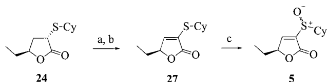
Scheme 8. Reagents and conditions: (a) m -CPBA, \text{CH}_2\text{Cl}_2 , 0 °C, 91%; (b) TFAA (2 equiv.), \text{CH}_2\text{Cl}_2 , 0 °C, 98%, ee : 99%; (c) m -CPBA, \text{CH}_2\text{Cl}_2 , 0 °C, 98%, dr 1:1.
