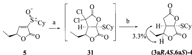
Scheme 11. Synthesis of an analog of ethisolide. Reagents and conditions: (a) \text{CCl}_3\text{COCl} , \text{Zn-Cu} , THF, 10 min, 0^\circ\text{C} ; (b) Raney nickel, EtOH, room temp., 48% (2 steps).
