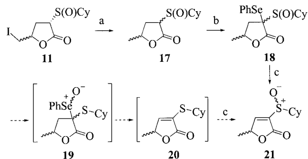
Scheme 5. Reagents and conditions: (a) \text{Bu}_3\text{SnH} , AIBN, THF, 65^{\circ}\text{C} , 97%; (b) LiHMDS, THF, -78^{\circ}\text{C} , then PhSeCl, 60 to 82%; (c) m -CPBA, pyridine, \text{CH}_2\text{Cl}_2 , 0^{\circ}\text{C} , 97%.
