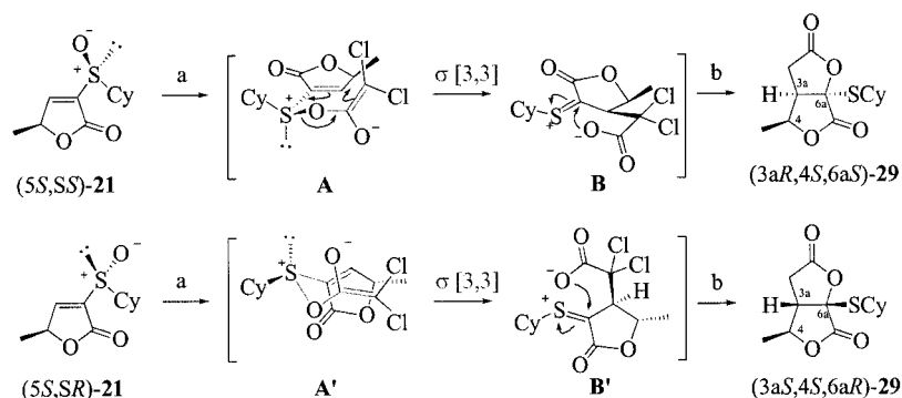
Scheme 10. Reagents and conditions: (a) \text{CCl}_3\text{COCl} , Zn-Cu, THF, 10 min, 0 °C; (b) \text{Bu}_3\text{SnH} , AIBN, toluene, 110 °C.
